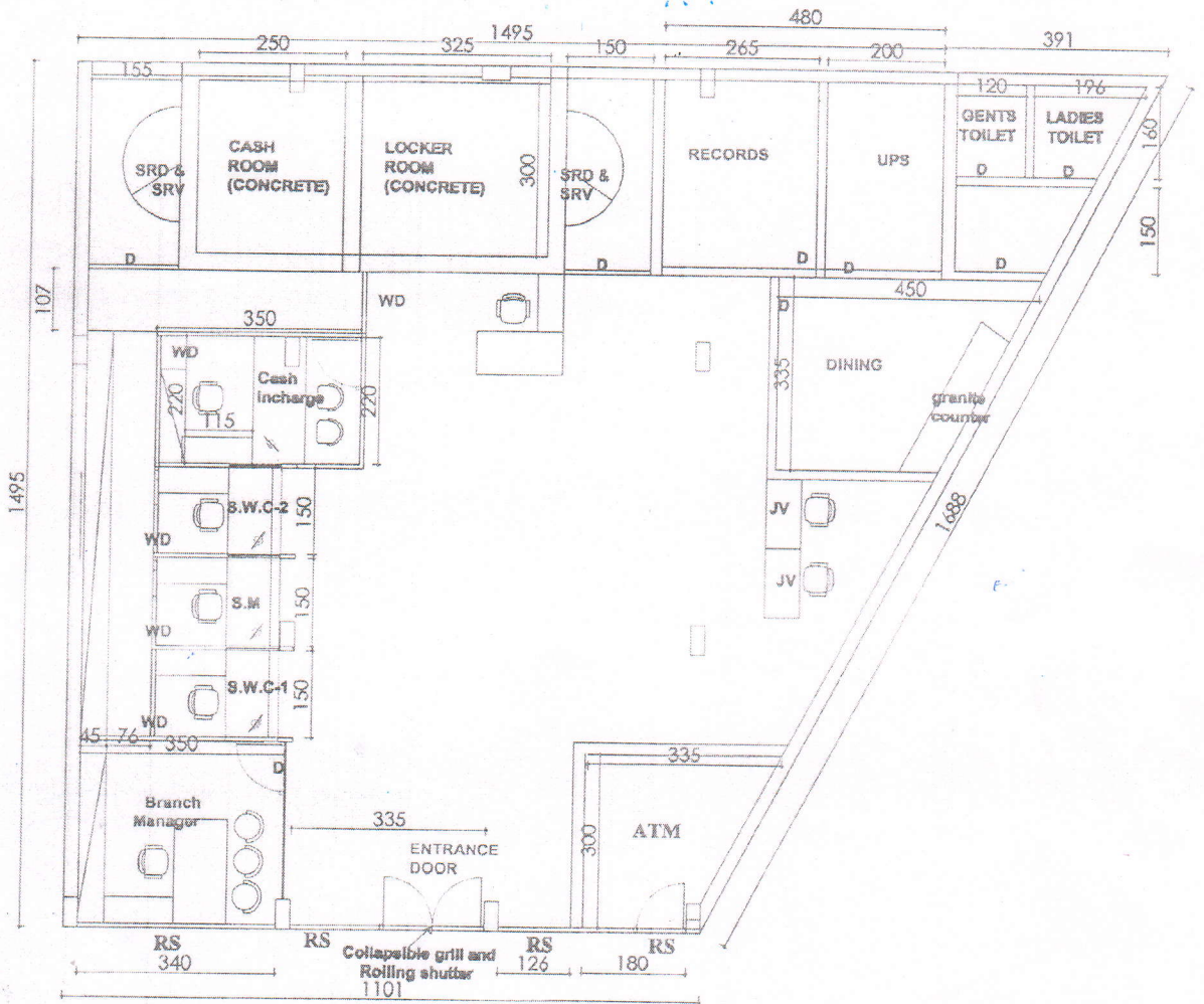
SBI NRI KILIMANOOR - NEW PREMISES -GROUND FLOOR - DWG NO.2 DT. 20.12.24 - Carpet area - 2403 Sft
